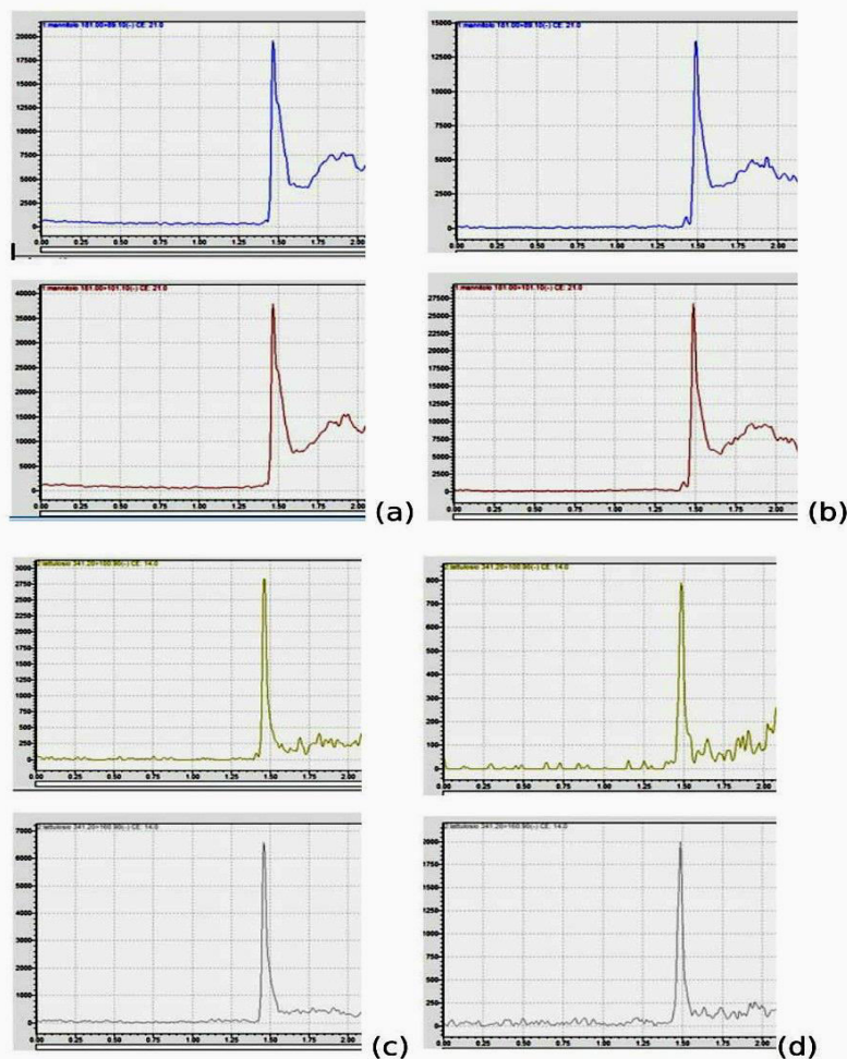
Fig. 2 (a) chromatograms of mannitol with standard addition. (b) chromatograms of mannitol without standard addition. (c) chromatograms of lactulose with standard addition. (d) chromatograms of lactulose without standard addition
